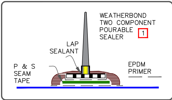
OPTION WITH PEEL & STICK SEAM TAPE ATTACHMENT
