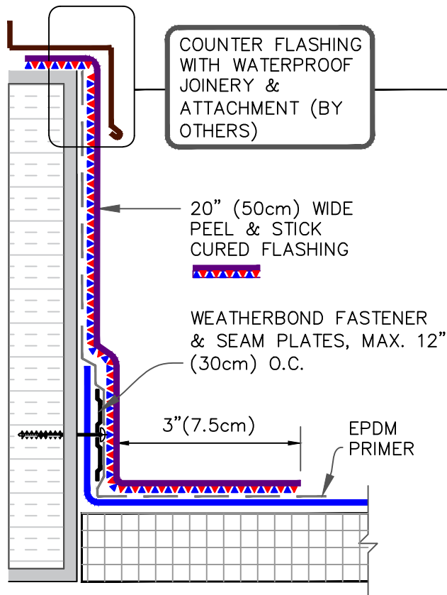
FASTENERS INTO CURB
