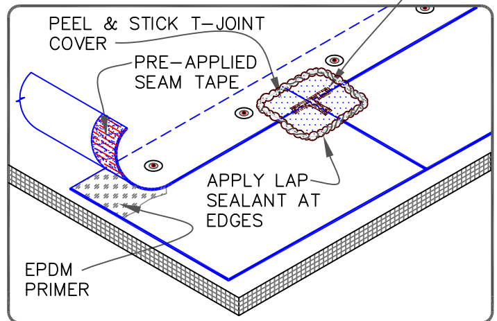
PRE-APPLIED SEAM TAPE
